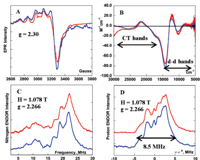
Figure 1. Overlay of reduced NiR with excess NO (red) and nitrite bound NiR (blue) (A) EPR, (B) MCD, (C) N 14 ENDOR, (D) H 1 ENDOR, with exchangeable features with 8.5 MHz coupling. Parts A and B have nitrite bound to T2 site with the T1 Cu reduced to remove intense overlapping T1 features. ENDOR data are collected at 1.078 T where there is no contribution from T1 Cu.
